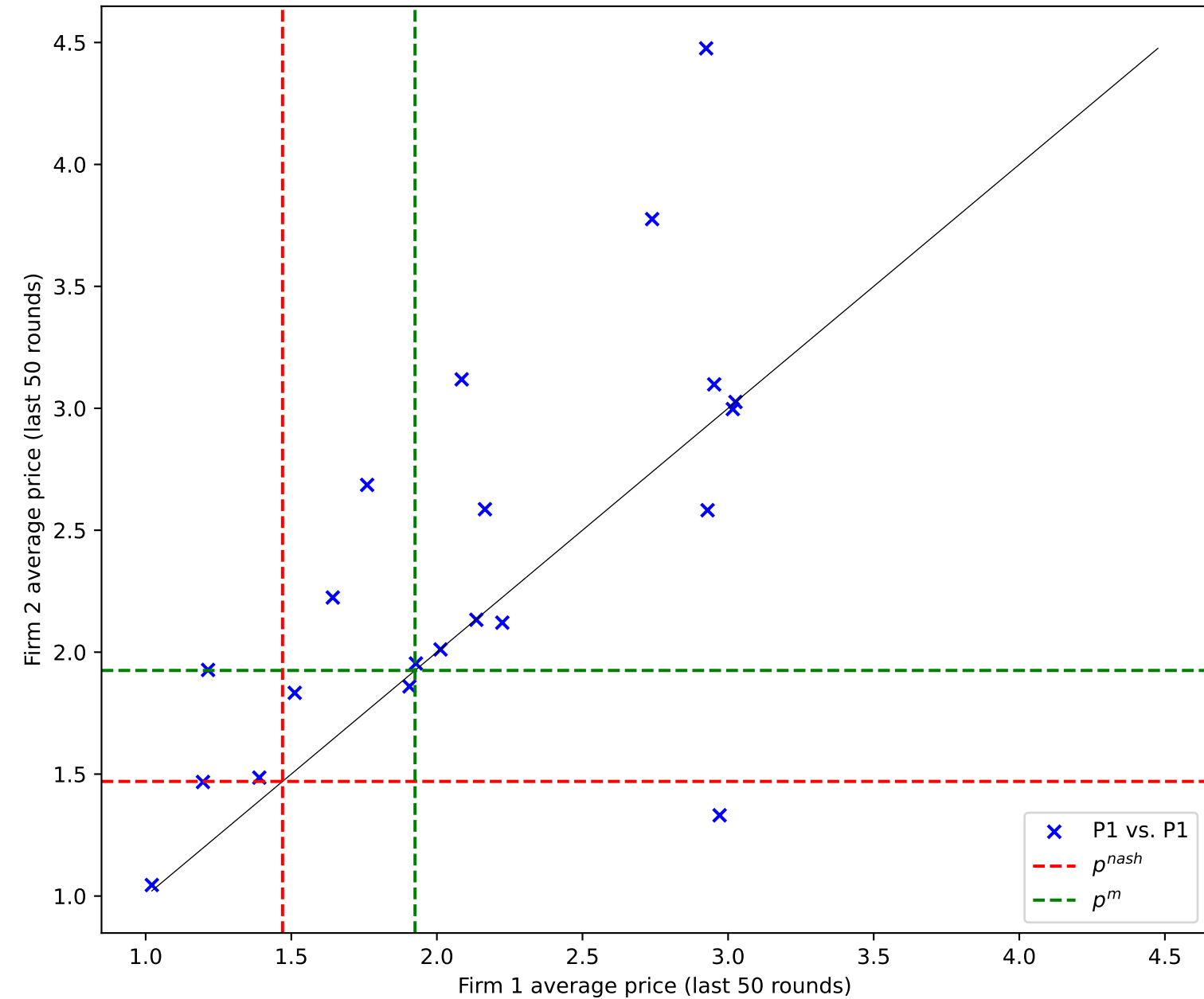
P1 vs P1: Pricing Behavior
