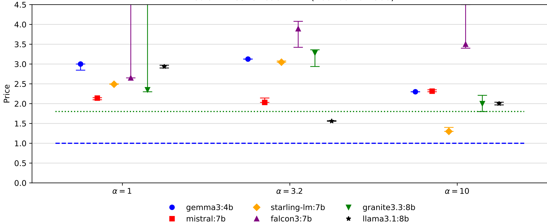
Median Price for each LLM (Rounds 201-300)
