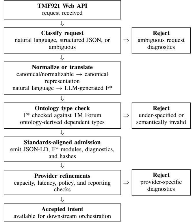
Fig. 1. Online TMF921 intent-admission pipeline. The standards-aligned gate checks whether the request is actionable under the ontology-derived dependent types; provider refinements then check local admissibility constraints.
