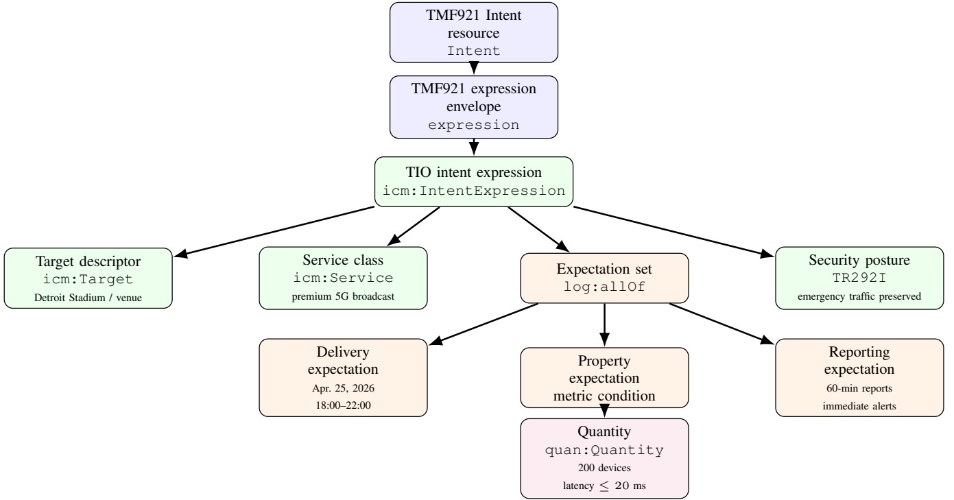
Fig. 2. TMF921/TIO ontology fragment for the Detroit Stadium intent. The nodes are standards-level concepts carried by the TMF921 intent resource and expression field; the small text shows demo values that inhabit those slots. Provider profiles and admission thresholds are not part of this ontology fragment.
