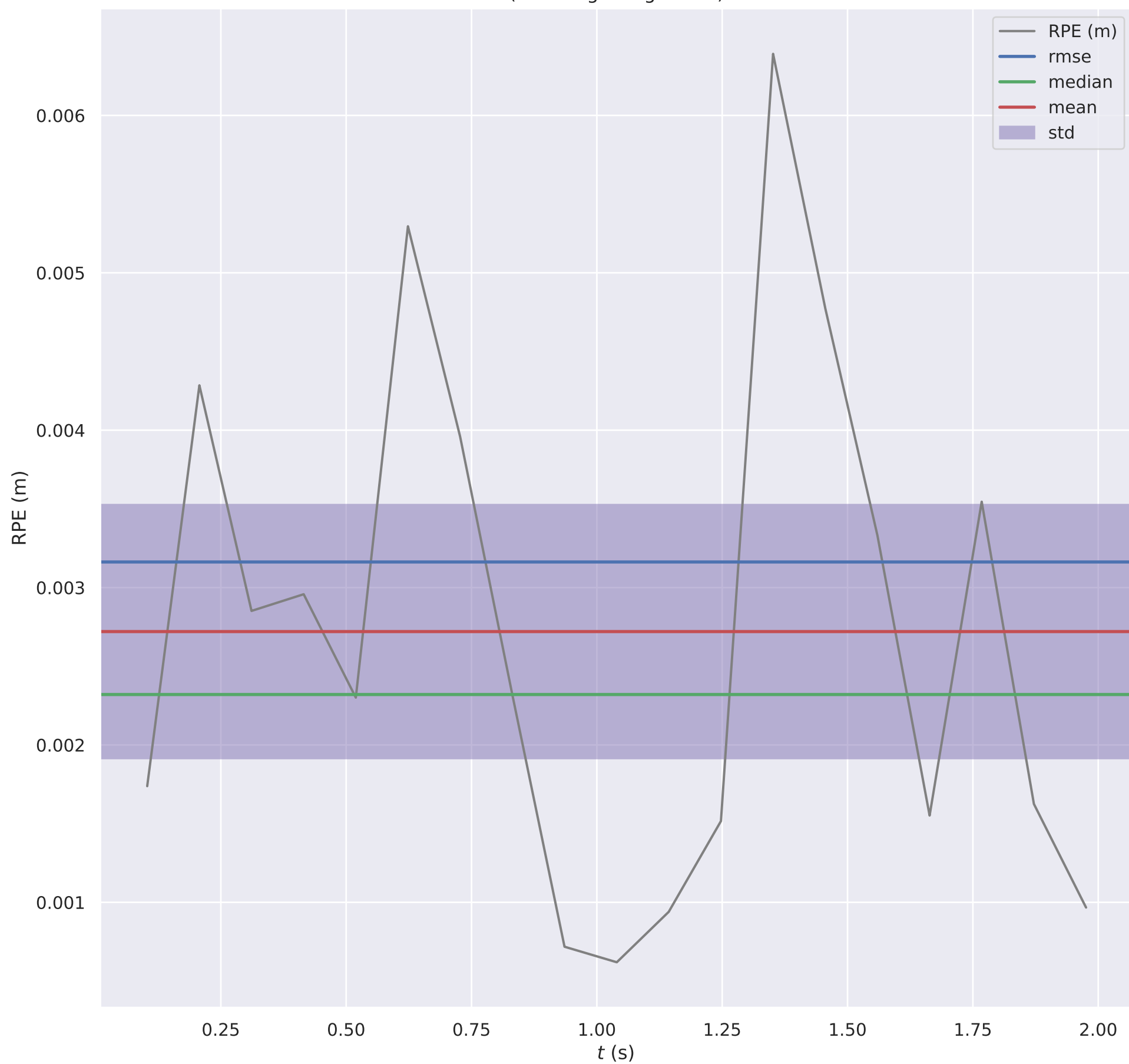
RPE w.r.t. translation part (m) for \delta = 1 (frames) using consecutive pairs (with origin alignment)
