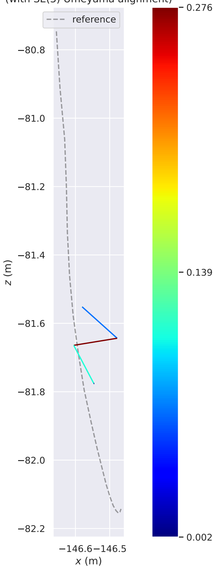
RPE w.r.t. translation part (m) for \delta = 1 (frames) using consecutive pairs (with SE(3) Umeyama alignment)
