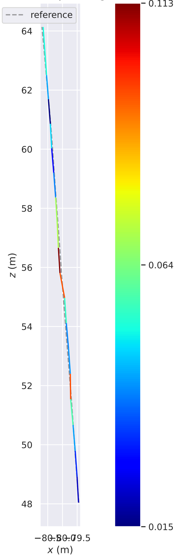
APE w.r.t. translation part (m) (with SE(3) Umeyama alignment)
