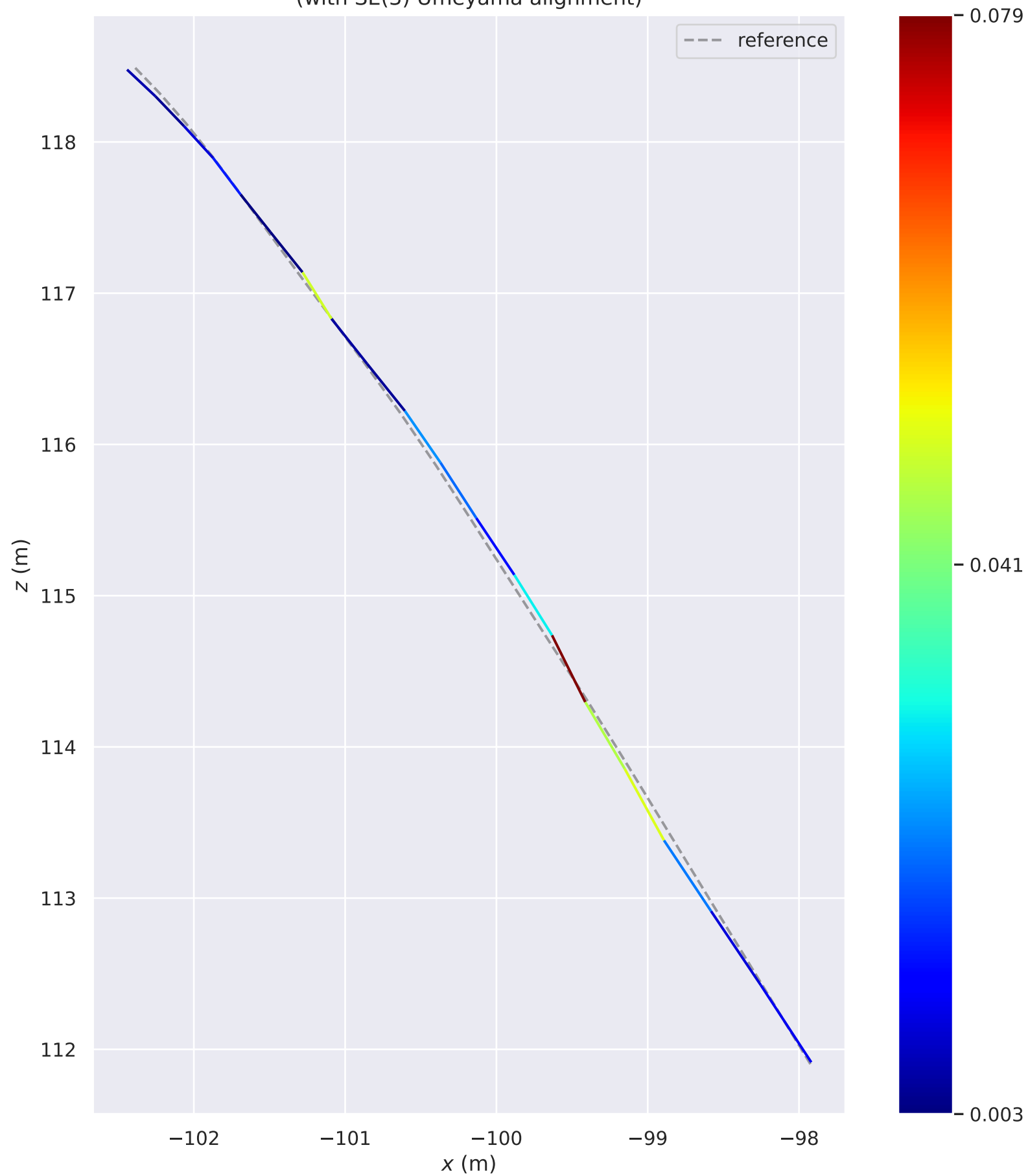
RPE w.r.t. translation part (m) for \delta = 1 (frames) using consecutive pairs (with SE(3) Umeyama alignment)
