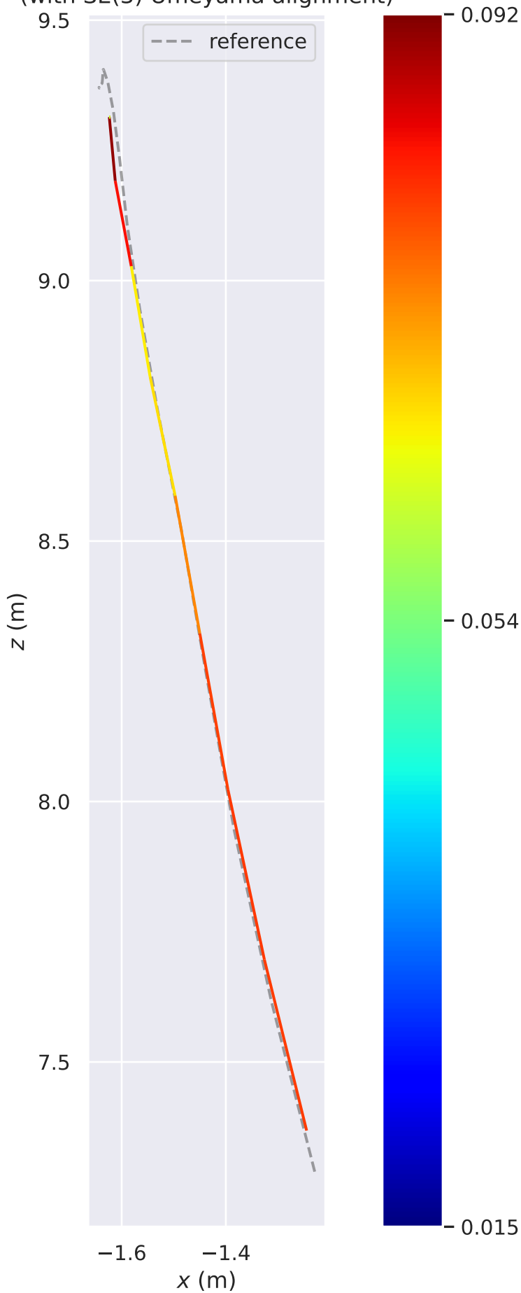
APE w.r.t. translation part (m) (with SE(3) Umeyama alignment)
