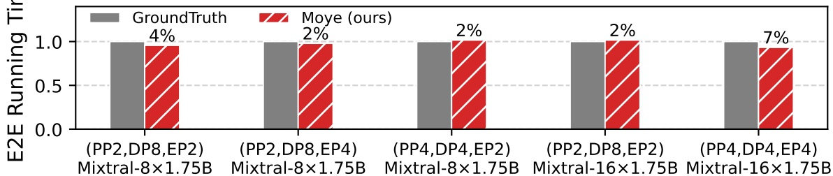
End-to-End Performance Comparison (MoE Models)
