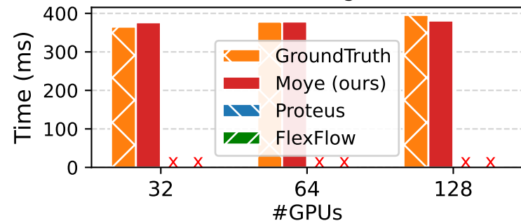
ResNet152
