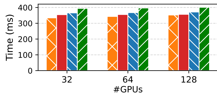
ResNet152
