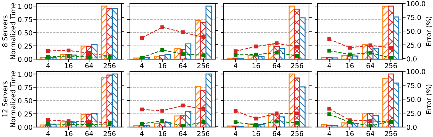
AllReduce (Ring)
