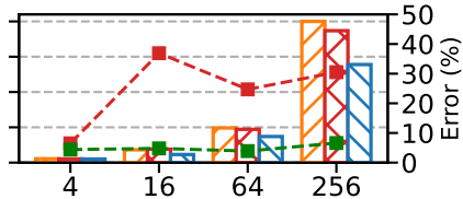
ReduceScatter
