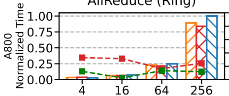
AllReduce (Ring)
