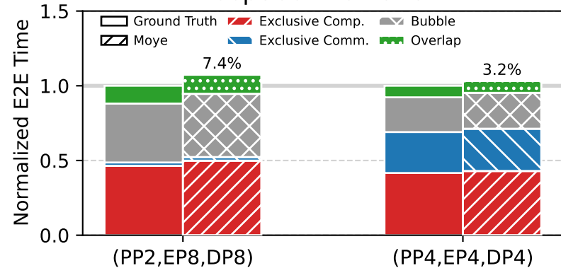
DeepSeek-V3 variant
