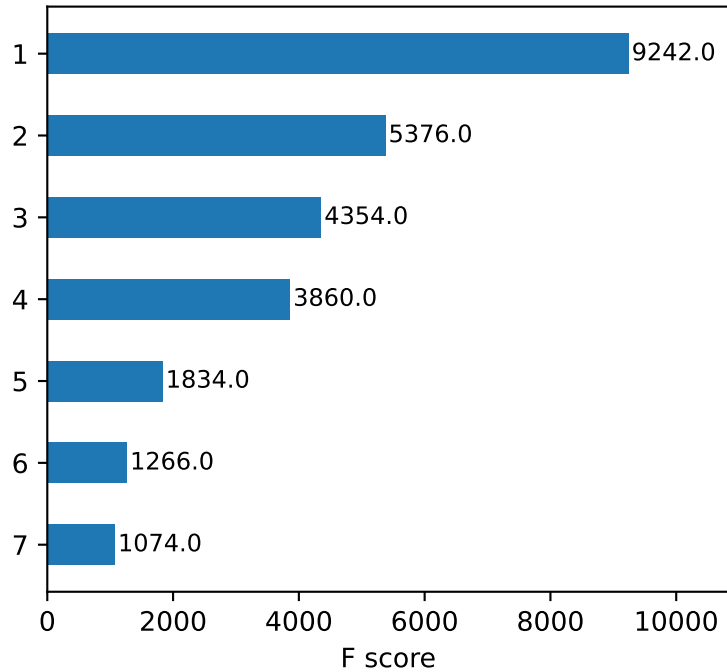
Feature Importance - RTX 3090
