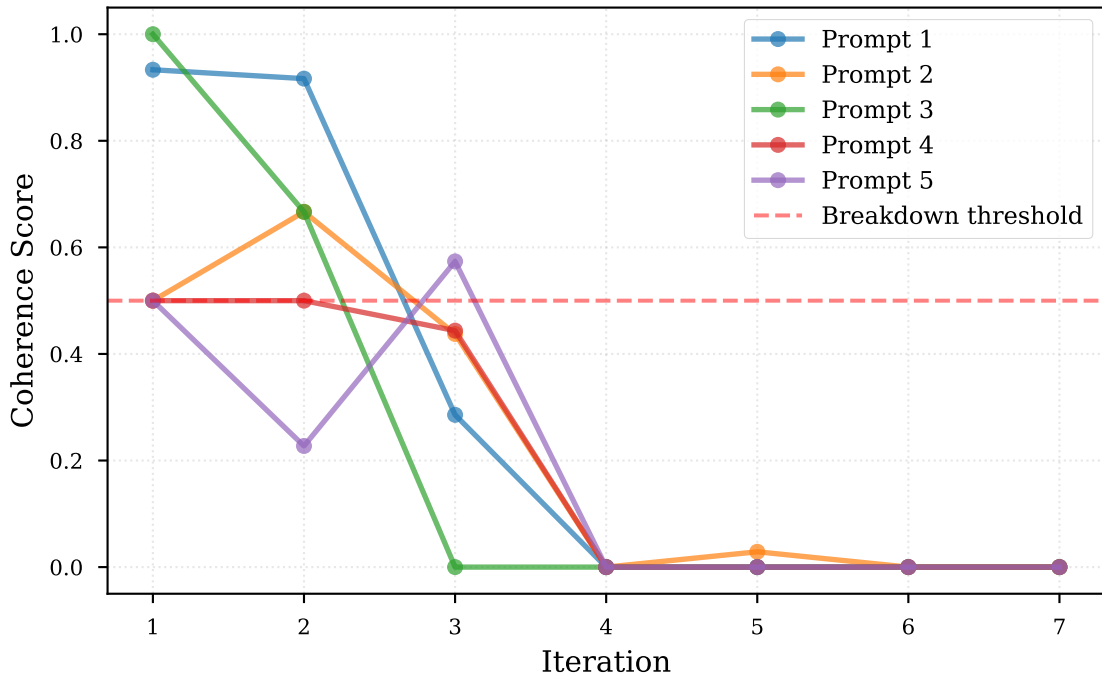
Coherence Degradation Over Attack Iterations
