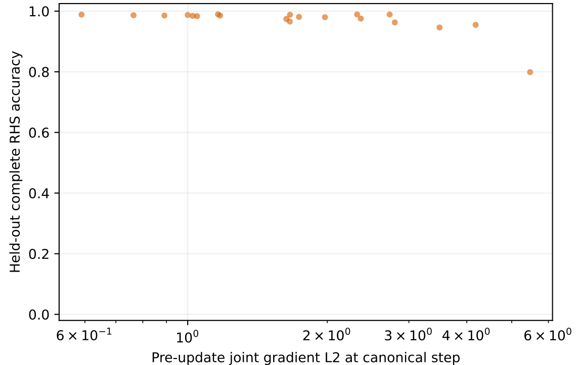
Immediate neighbors of later canonical failures: 20 supported triplets Descriptions of observed trajectories; association does not establish a cause
