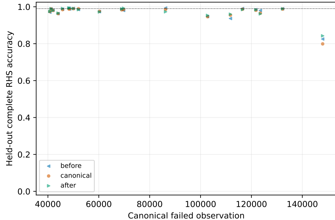
Immediate neighbors of later canonical failures: 20 supported triplets Descriptions of observed trajectories; association does not establish a cause
