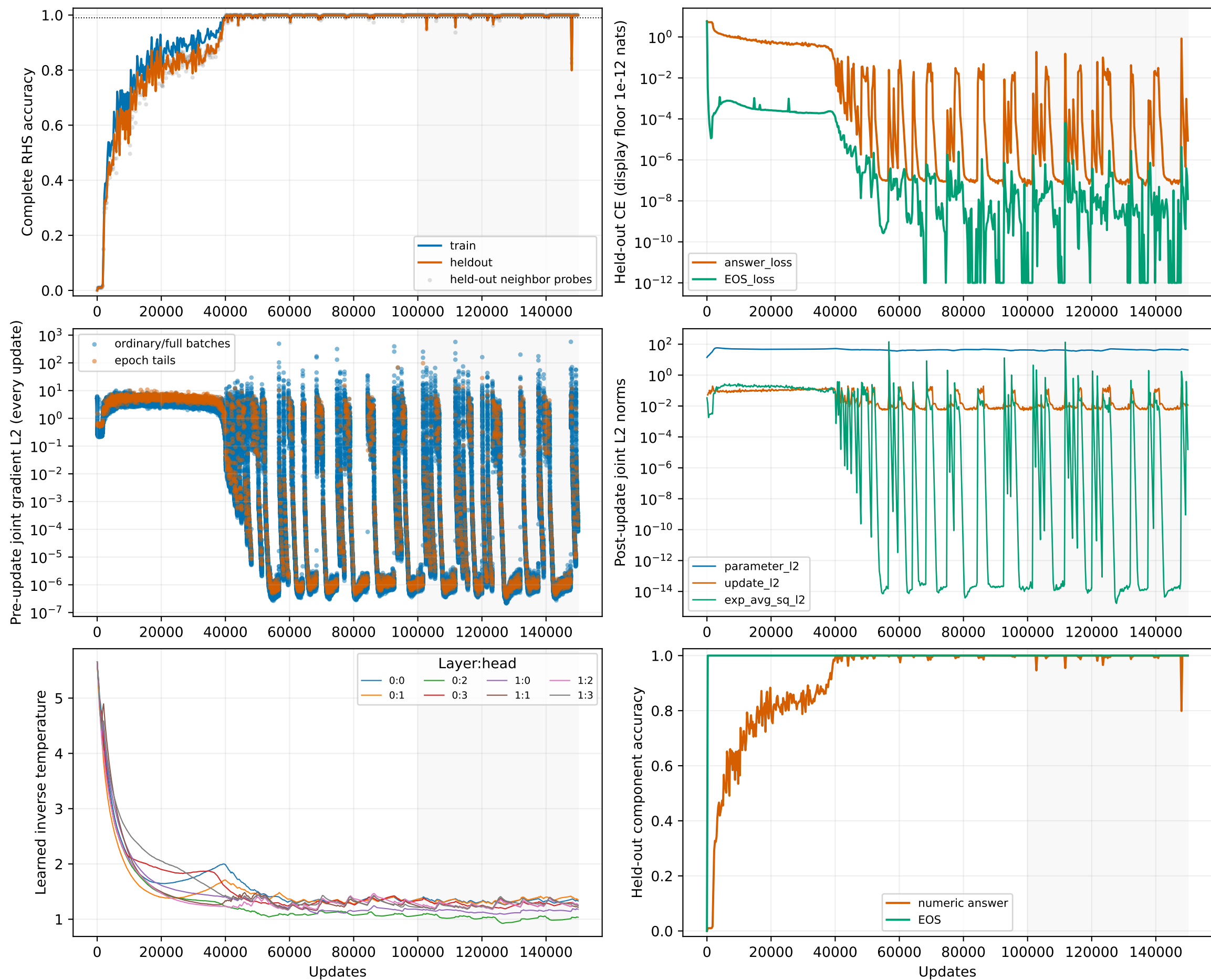
adamw-mod193-lr001: AdamW / GPTMini lr=0.001, short_final; complete 150,000-update calibration Gray band: prospectively scored final tail
