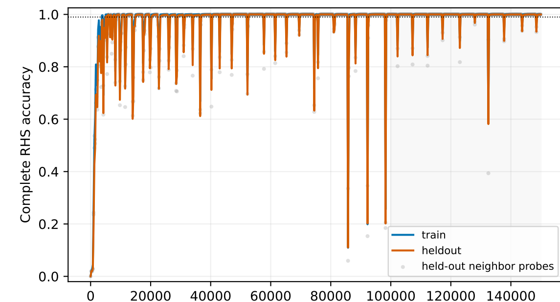
short-lr001: raw AMSGradW / GPTMini, lr=0.001, short_final Complete 150,000-update calibration; gray band is prospectively scored final tail
