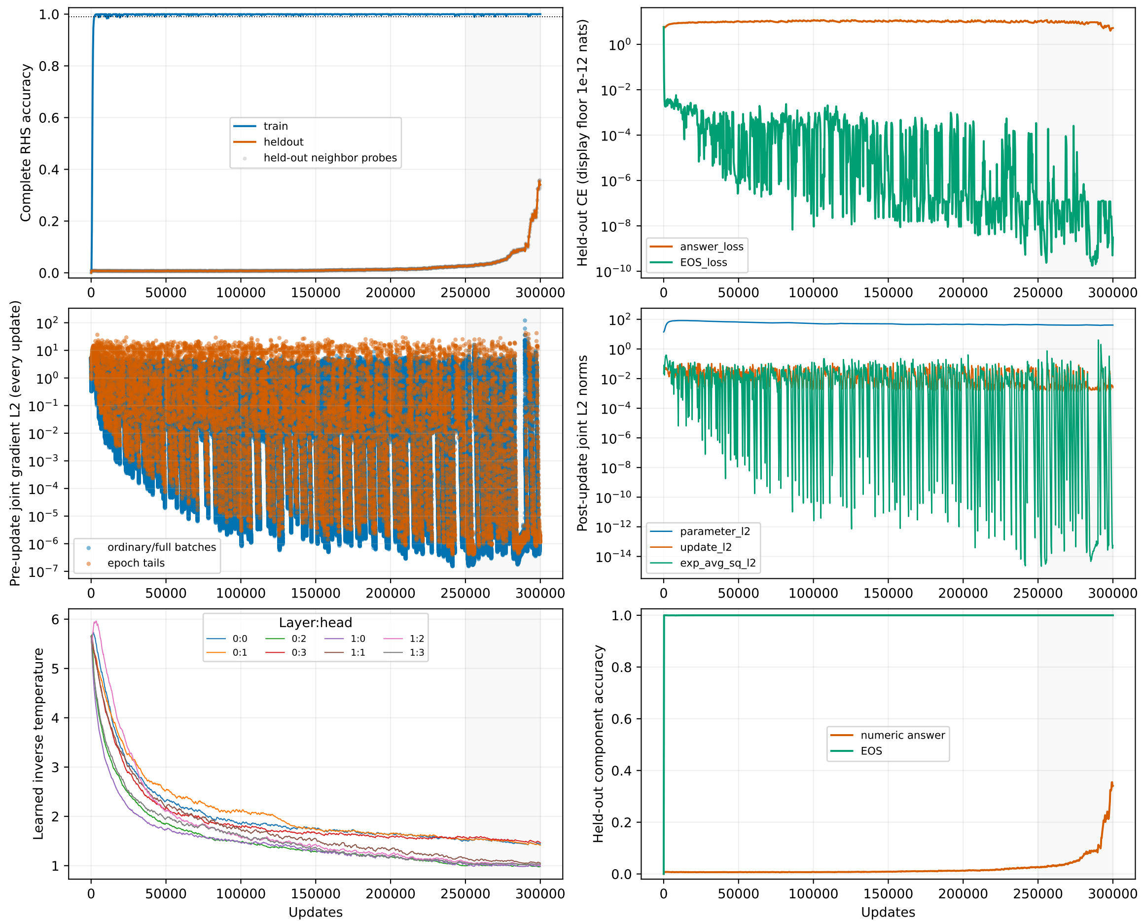
adamw-sparsemax: AdamW / GPTMini lr=0.0003, short_final; complete 300,000-update calibration Gray band: prospectively scored final tail
