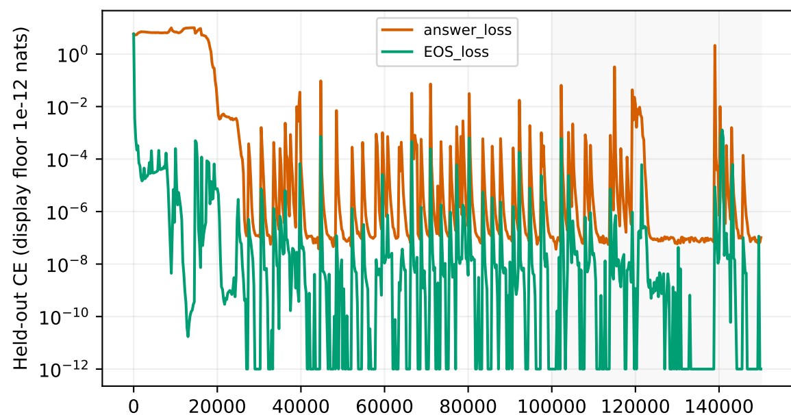
adamw-mod193-fraction25-lr001: AdamW / GPTMini lr=0.001, short_final; complete 150,000-update calibration Gray band: prospectively scored final tail
