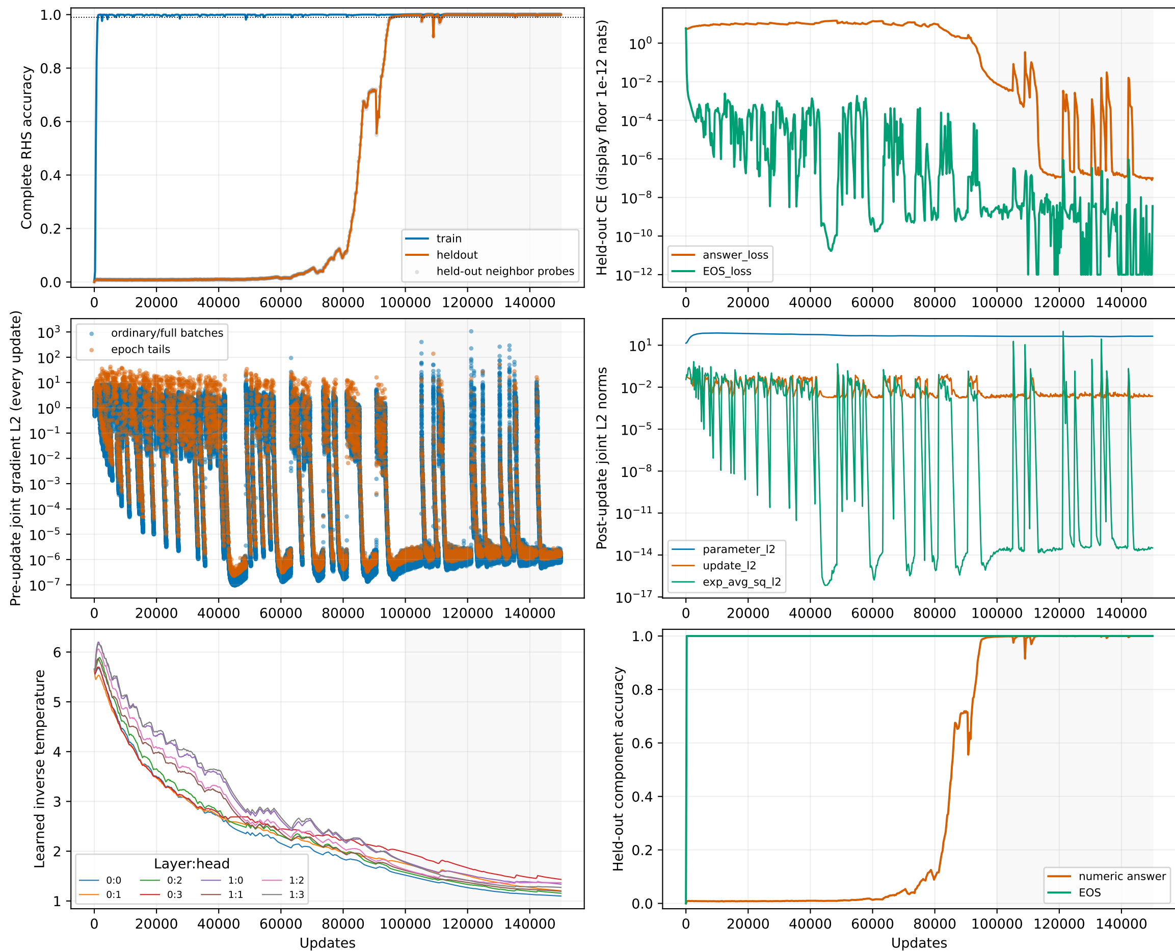
adamw-mod193-fraction25-lr0003: AdamW / GPTMini lr=0.0003, short_final; complete 150,000-update calibration Gray band: prospectively scored final tail
