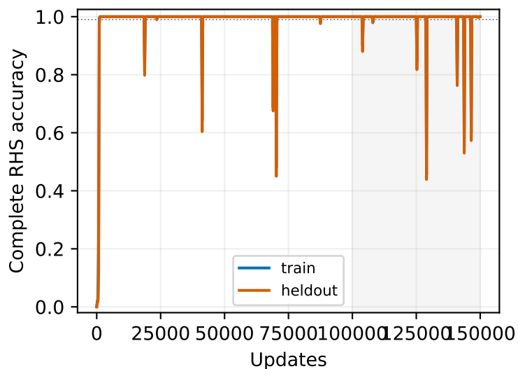
adamw-short-lr001
