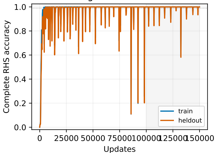
amsgradw-short-lr001
