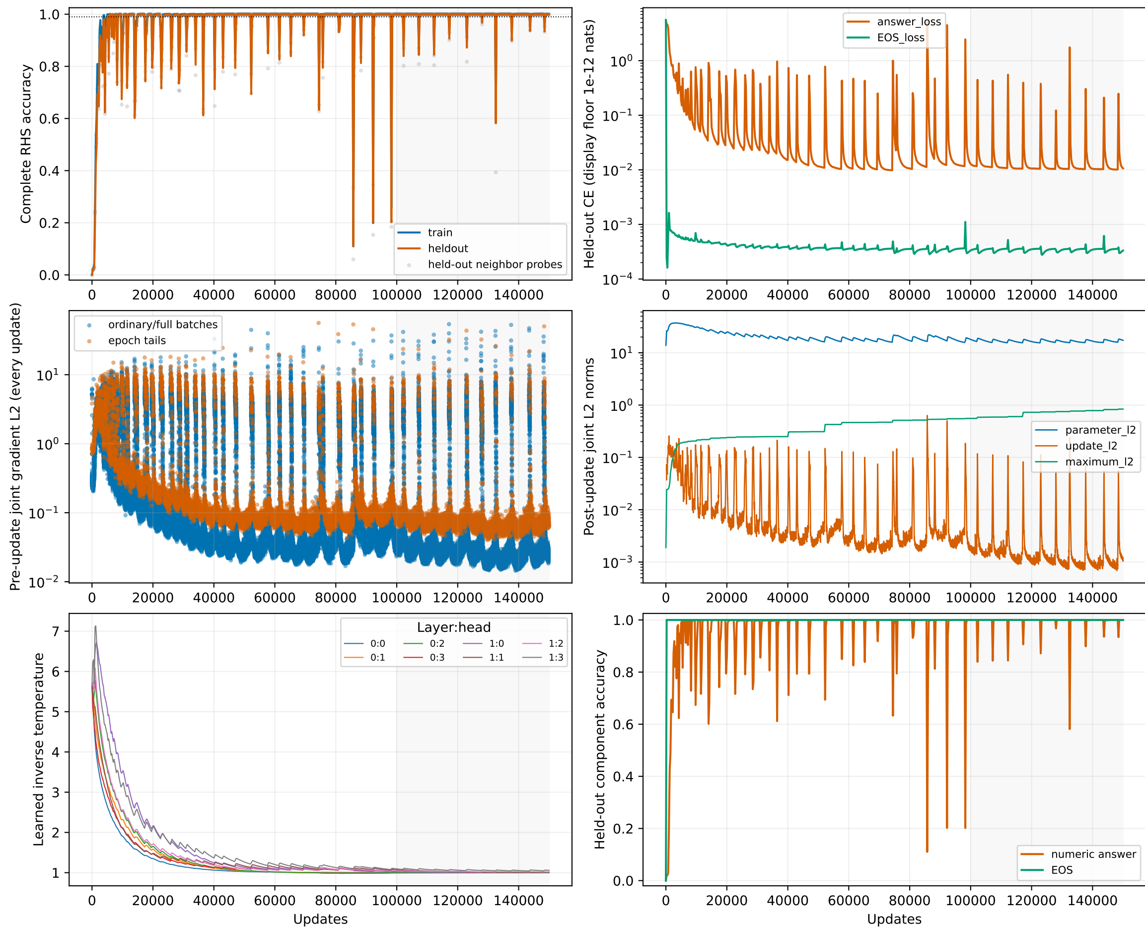
amsgradw-short-lr001: raw AMSGradW / GPTMini lr=0.001, short_final; complete 150,000-update calibration Gray band: prospectively scored final tail
