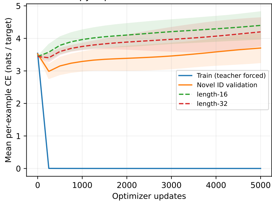
copy-repeat: 3 initialization seeds
