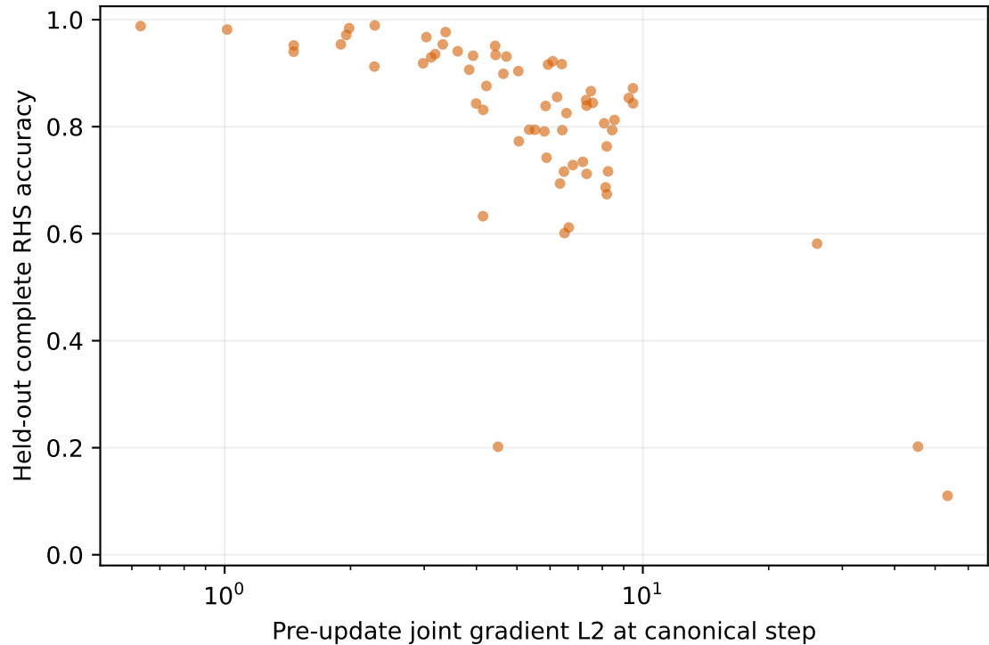
Immediate neighbors of later canonical failures: 64 supported triplets Descriptions of observed trajectories; association does not establish a cause
