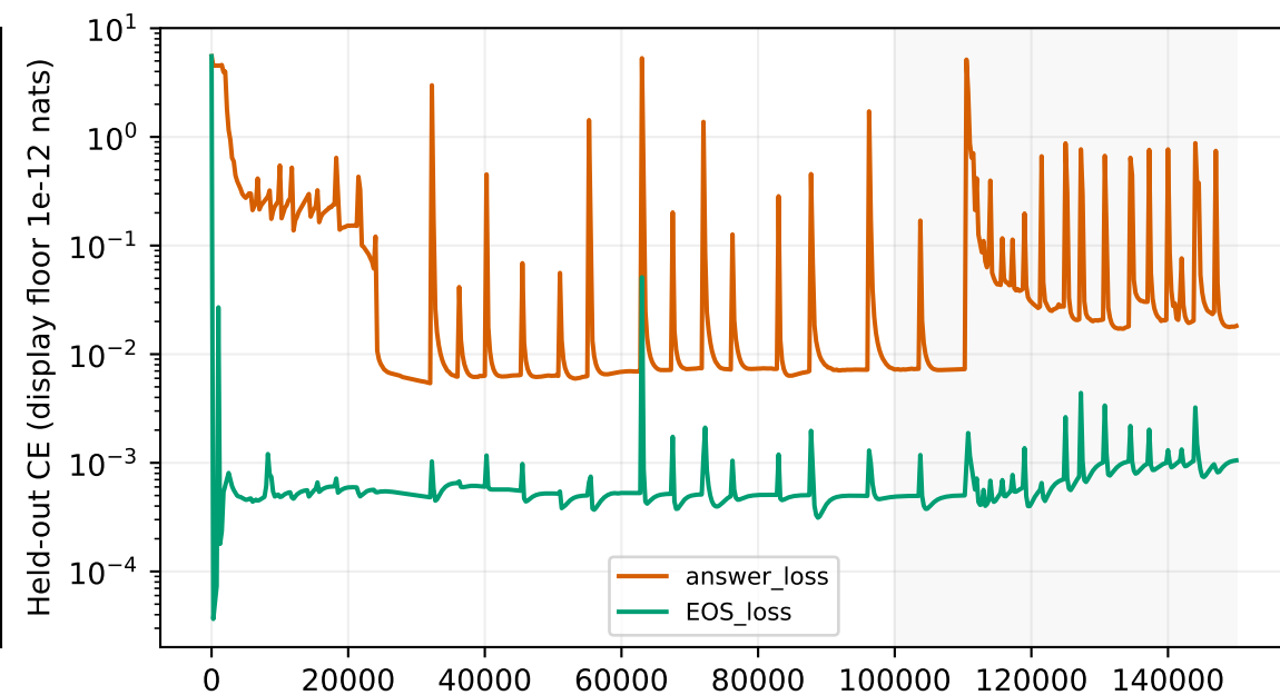
wrap-lr001: raw AMSGradW / GPTMini, lr=0.001, wrap_epoch Complete 150,000-update calibration; gray band is prospectively scored final tail
