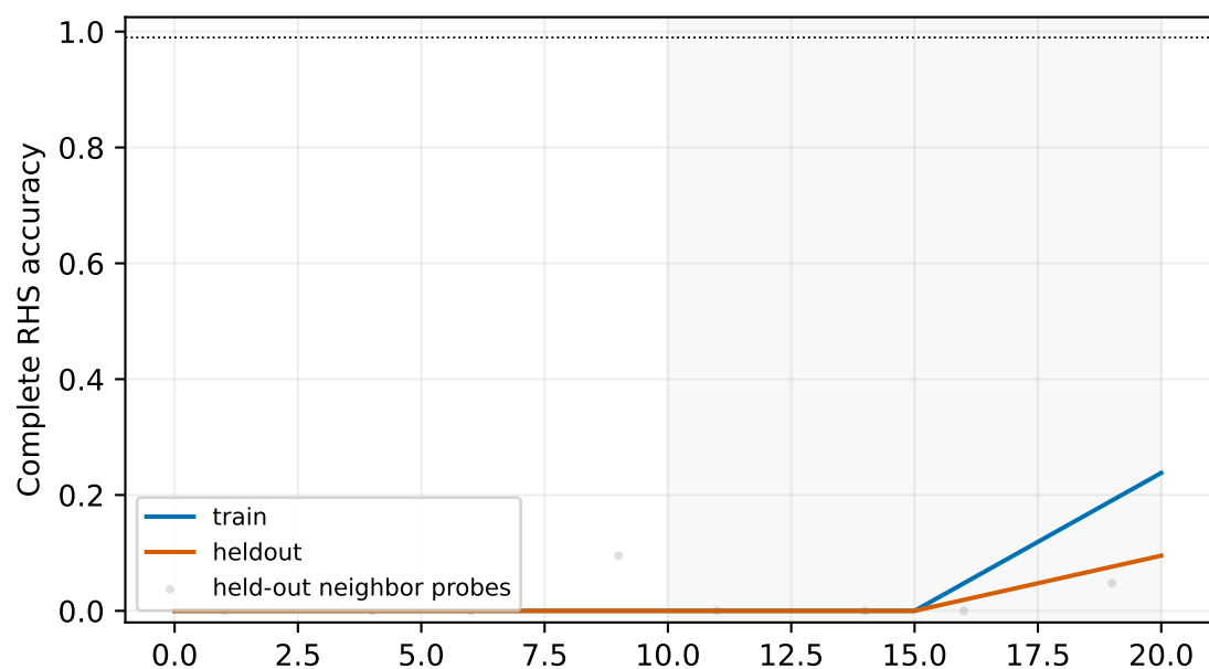
adamw-sparsemax: AdamW / GPTMini lr=0.0003, short_final; complete 20-update calibration Gray band: prospectively scored final tail
