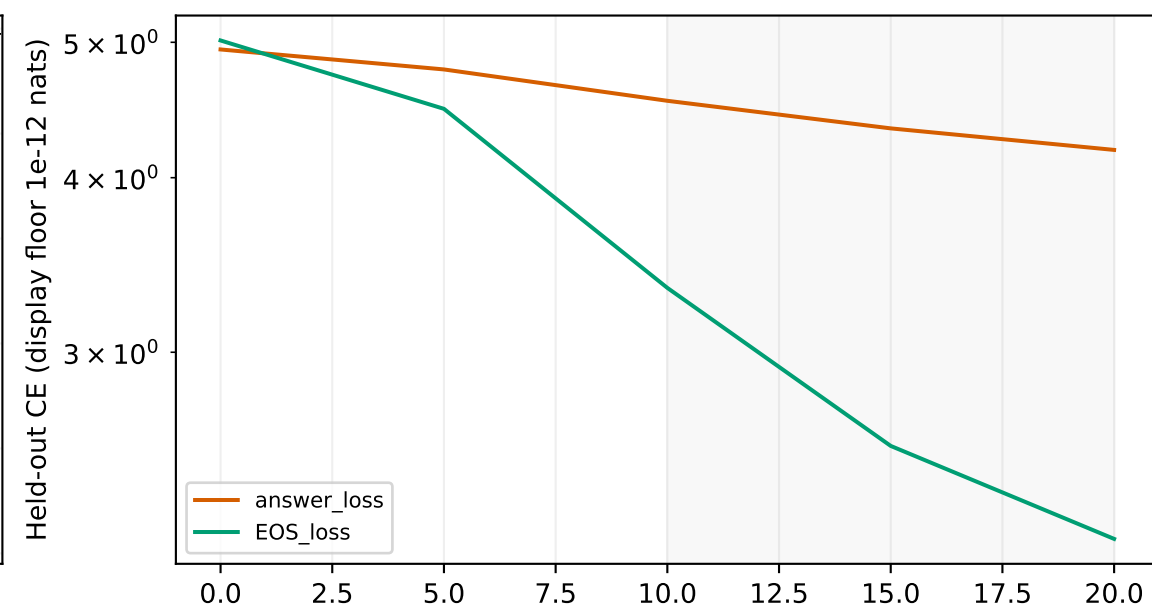
adamw-sparsemax: AdamW / GPTMini lr=0.0003, short_final; complete 20-update calibration Gray band: prospectively scored final tail
