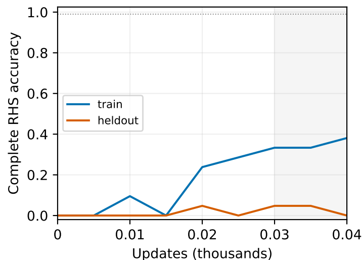
adamw-cosine-tail
