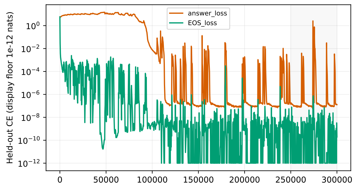
adamw-softmax: AdamW / GPTMini lr=0.0003, short_final; complete 300,000-update calibration Gray band: prospectively scored final tail
