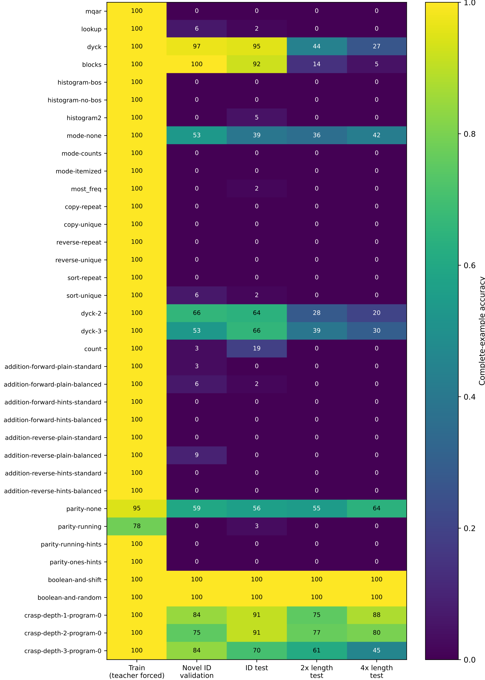
AMSGradW + softmax GPTMini: 37 variants, 1,000 updates, seed 0 Final checkpoint; hard-carry/position probes are in the JSON/CSV reports
