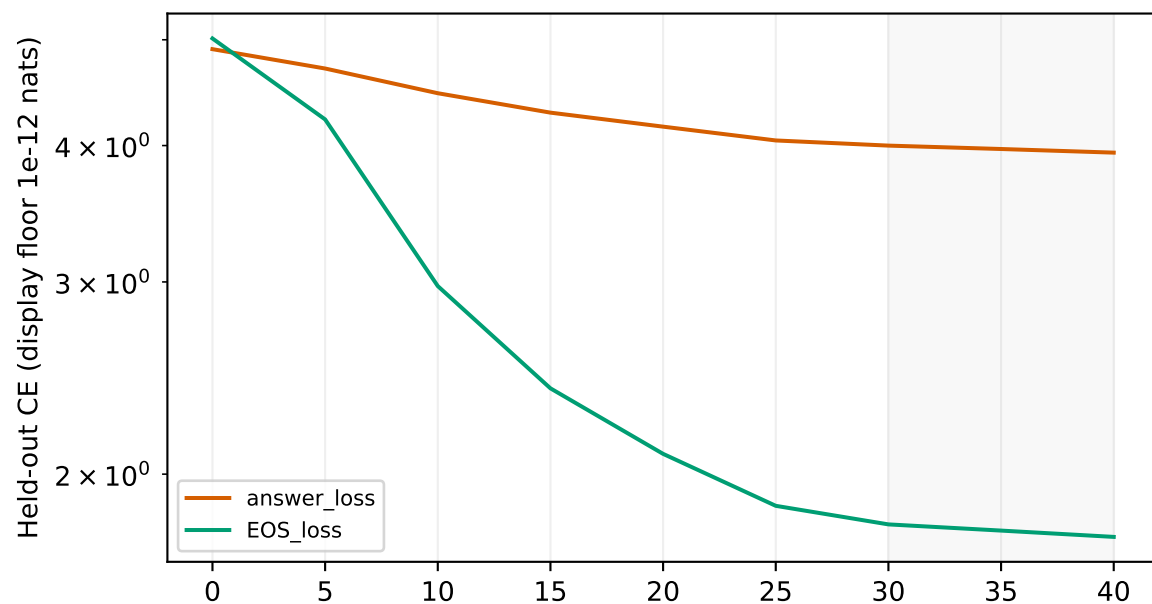
adamw-cosine-tail: AdamW / GPTMini lr=0.0003, short_final; complete 40-update calibration Gray band: prospectively scored final tail
