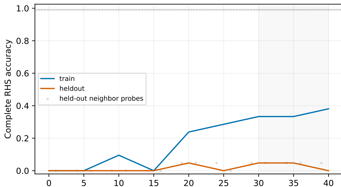
adamw-cosine-tail: AdamW / GPTMini lr=0.0003, short_final; complete 40-update calibration Gray band: prospectively scored final tail
