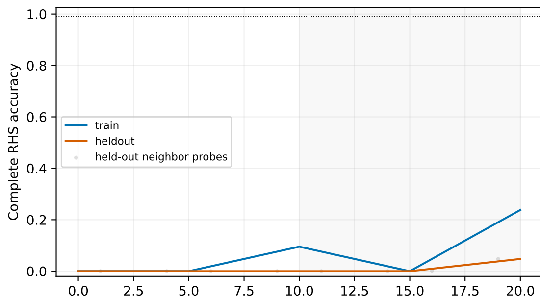
adamw-softmax: AdamW / GPTMini lr=0.0003, short_final; complete 20-update calibration Gray band: prospectively scored final tail
