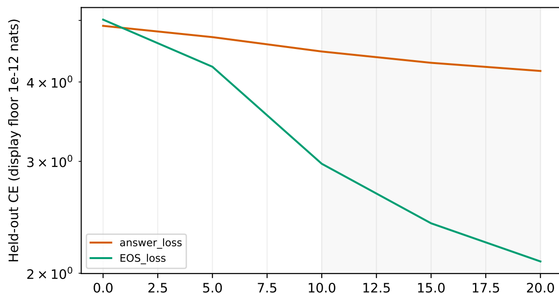
adamw-softmax: AdamW / GPTMini lr=0.0003, short_final; complete 20-update calibration Gray band: prospectively scored final tail
