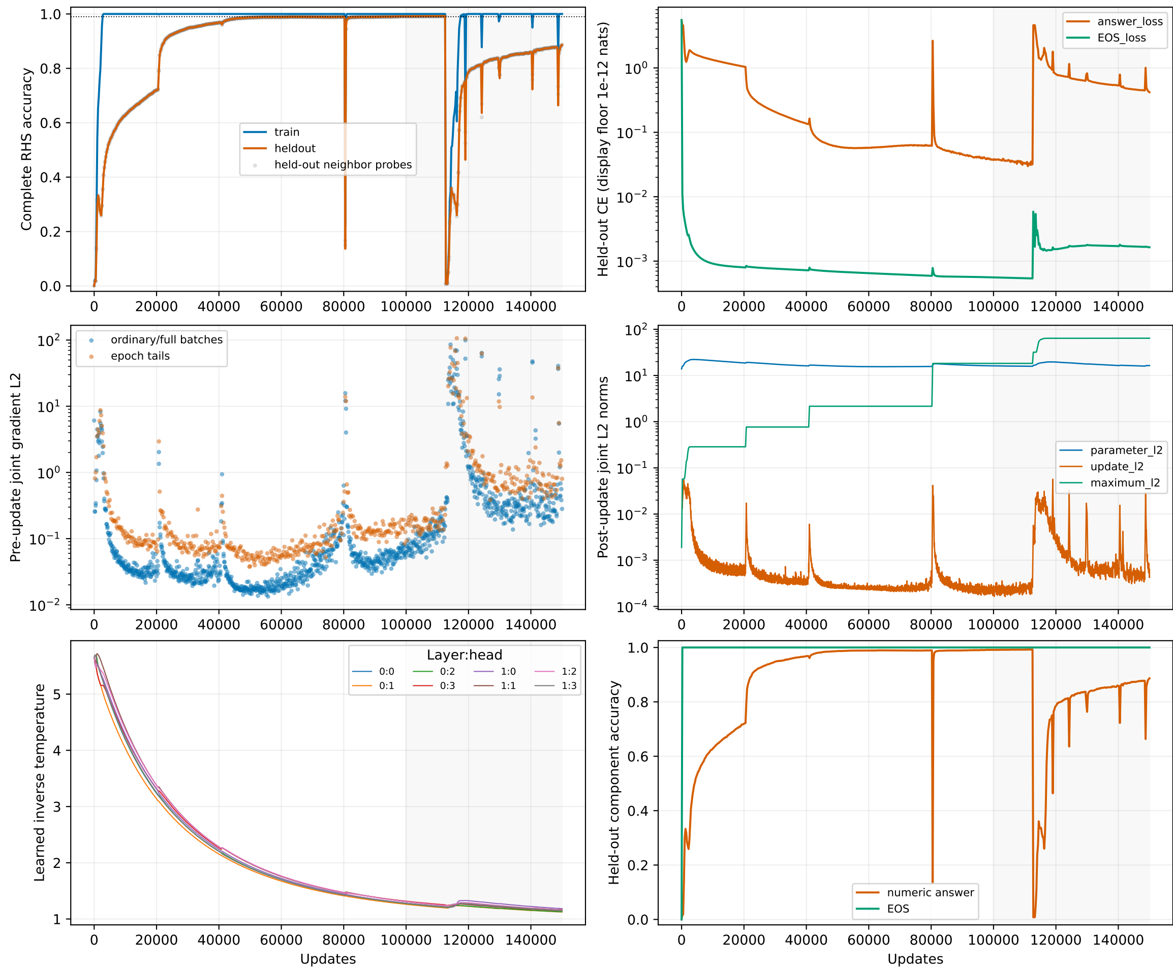
short-lr0002: raw AMSGradW / GPTMini, lr=0.0002, short_final Complete 150,000-update calibration; gray band is prospectively scored final tail
