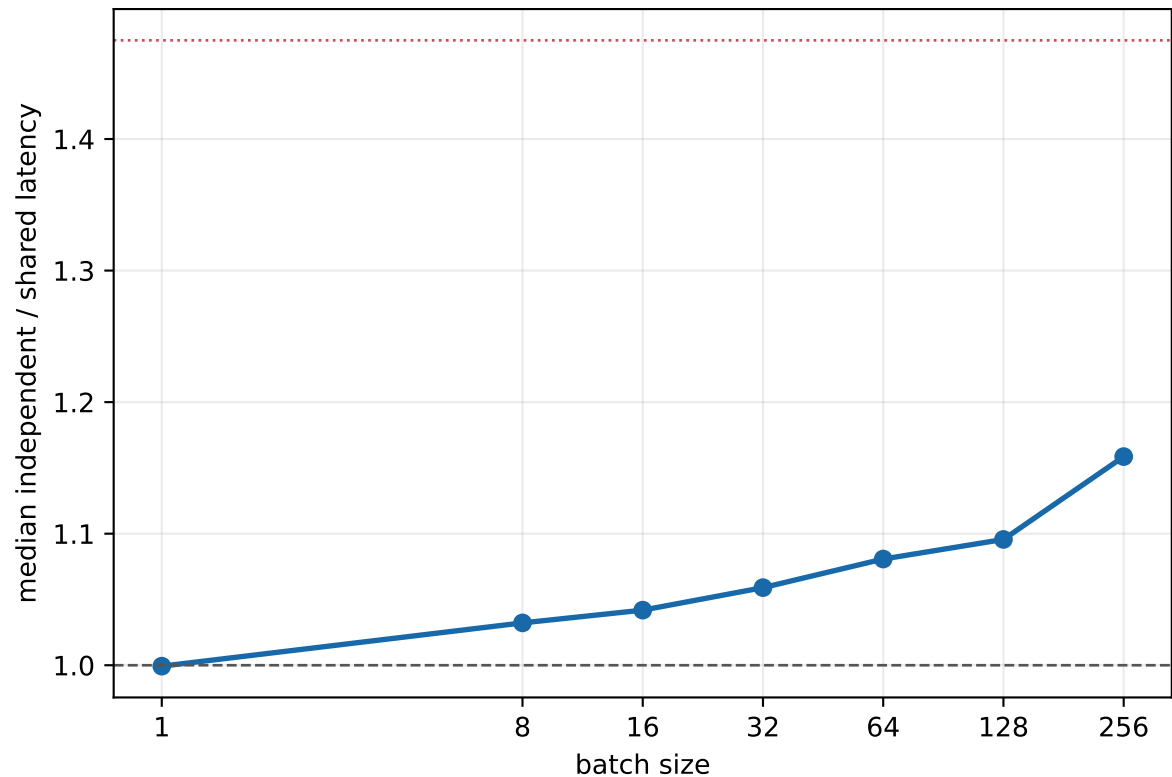
Performance value of shared selected KV in native decode
