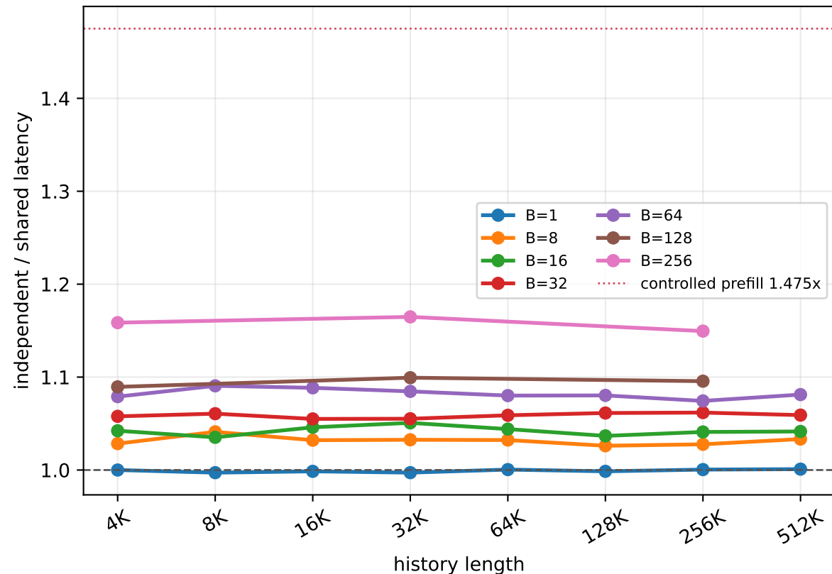
Performance value of shared selected KV in native decode
