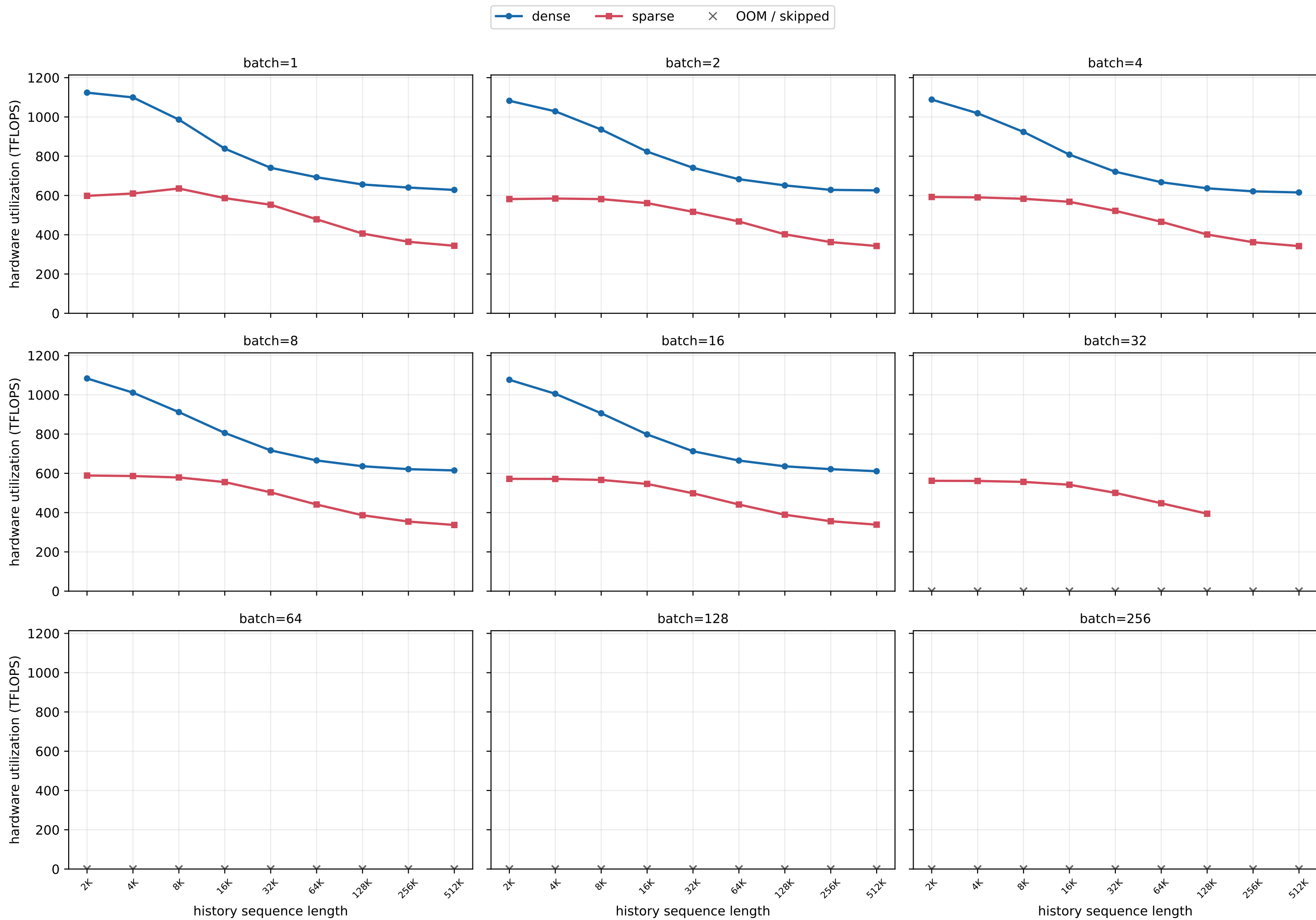
H800 MLA history scaling · new length=16K (chunked prefill) · ECHO Fig. 2 convention
