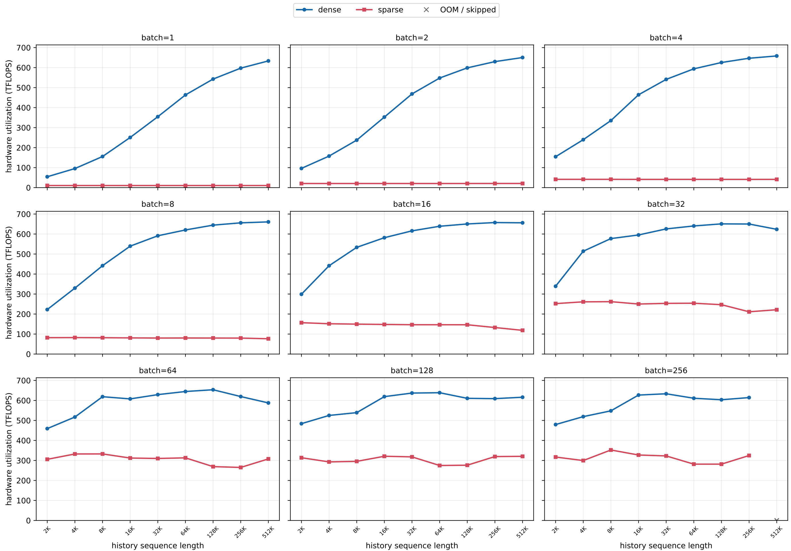
H800 MLA history scaling · new length=2 (chunked prefill) · ECHO Fig. 2 convention
