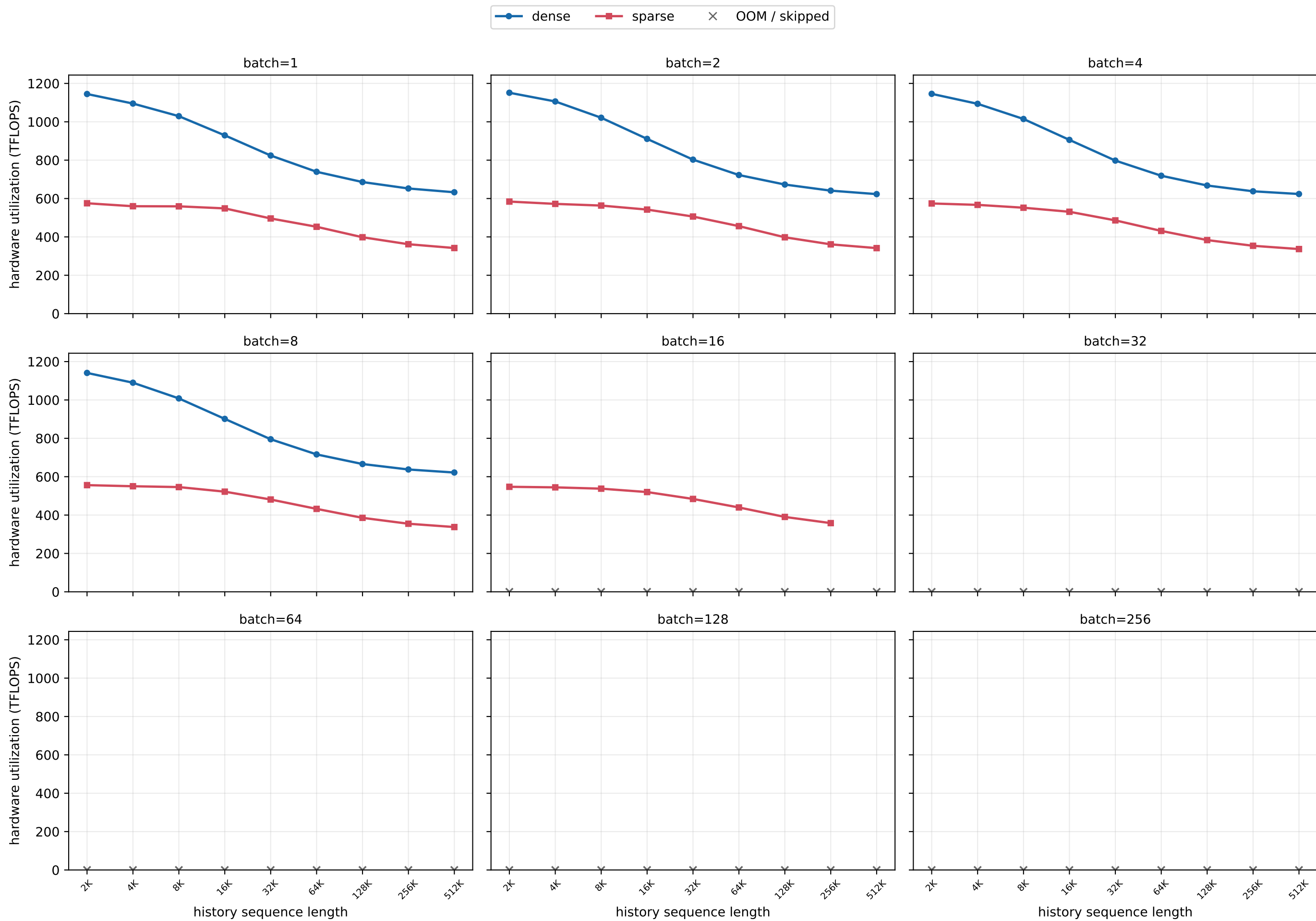
H800 MLA history scaling · new length=32K (chunked prefill) · ECHO Fig. 2 convention
