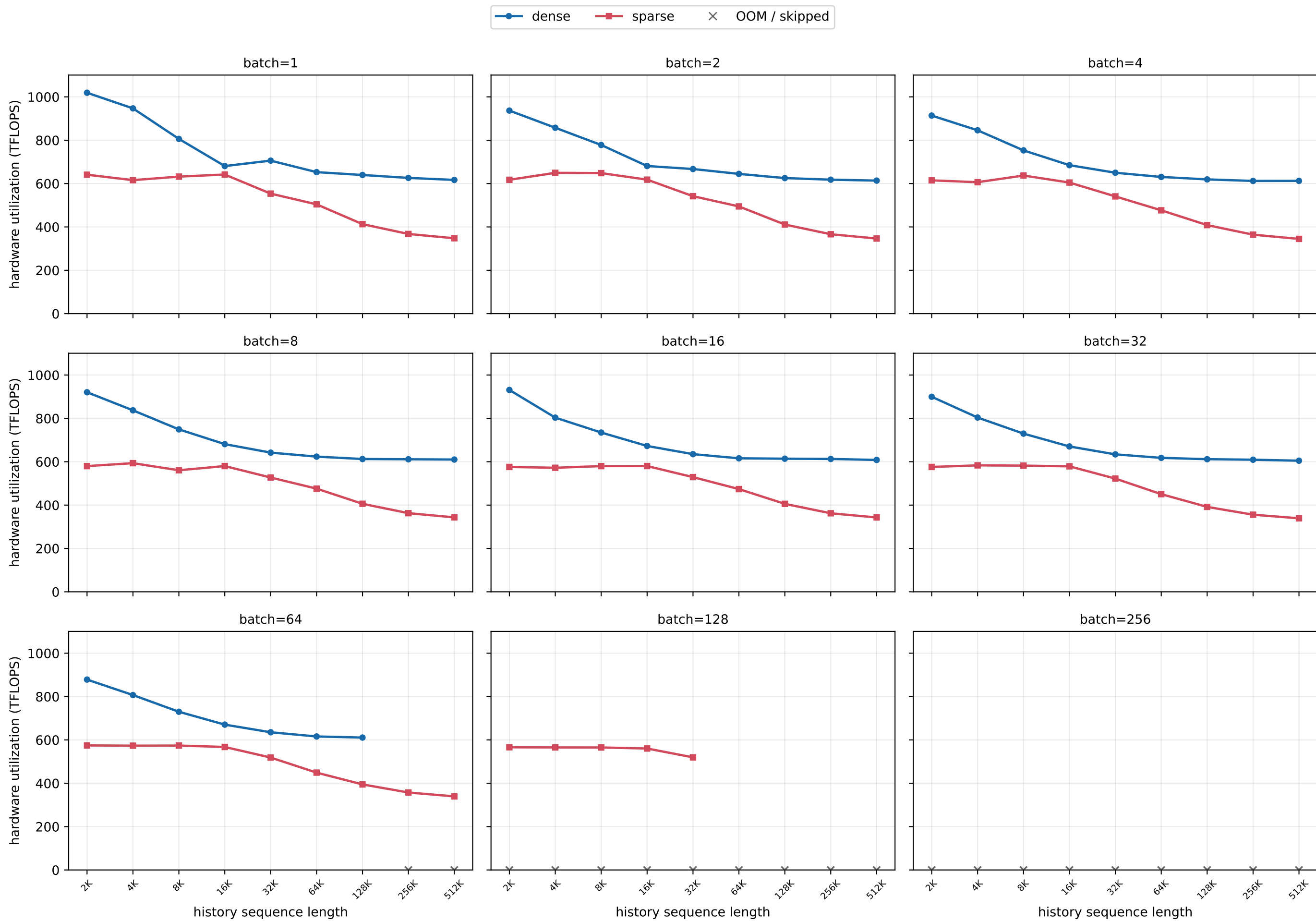
H800 MLA history scaling · new length=4K (chunked prefill) · ECHO Fig. 2 convention
