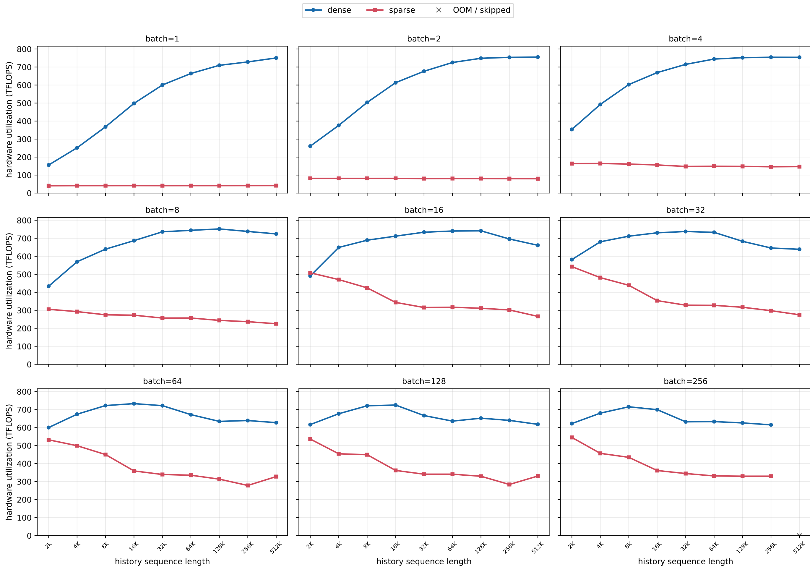
H800 MLA history scaling · new length=8 (chunked prefill) · ECHO Fig. 2 convention
