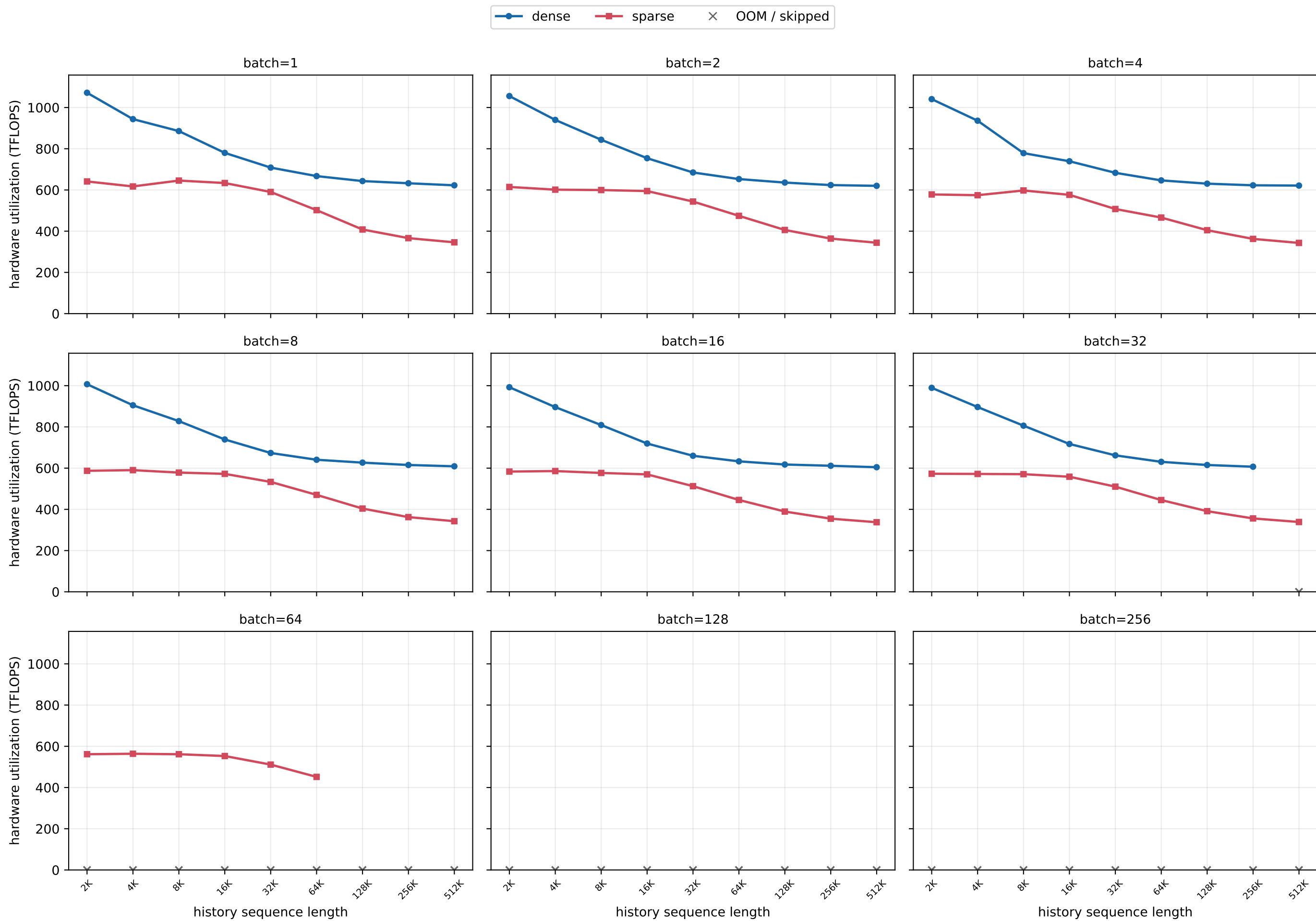
H800 MLA history scaling · new length=8K (chunked prefill) · ECHO Fig. 2 convention
