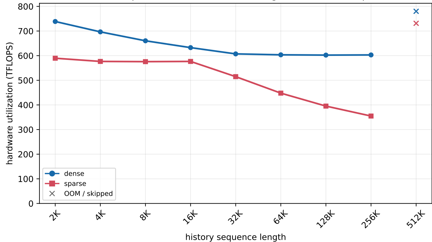
H800 MLA prefill - batch=128, new length=1K (chunked prefill)
