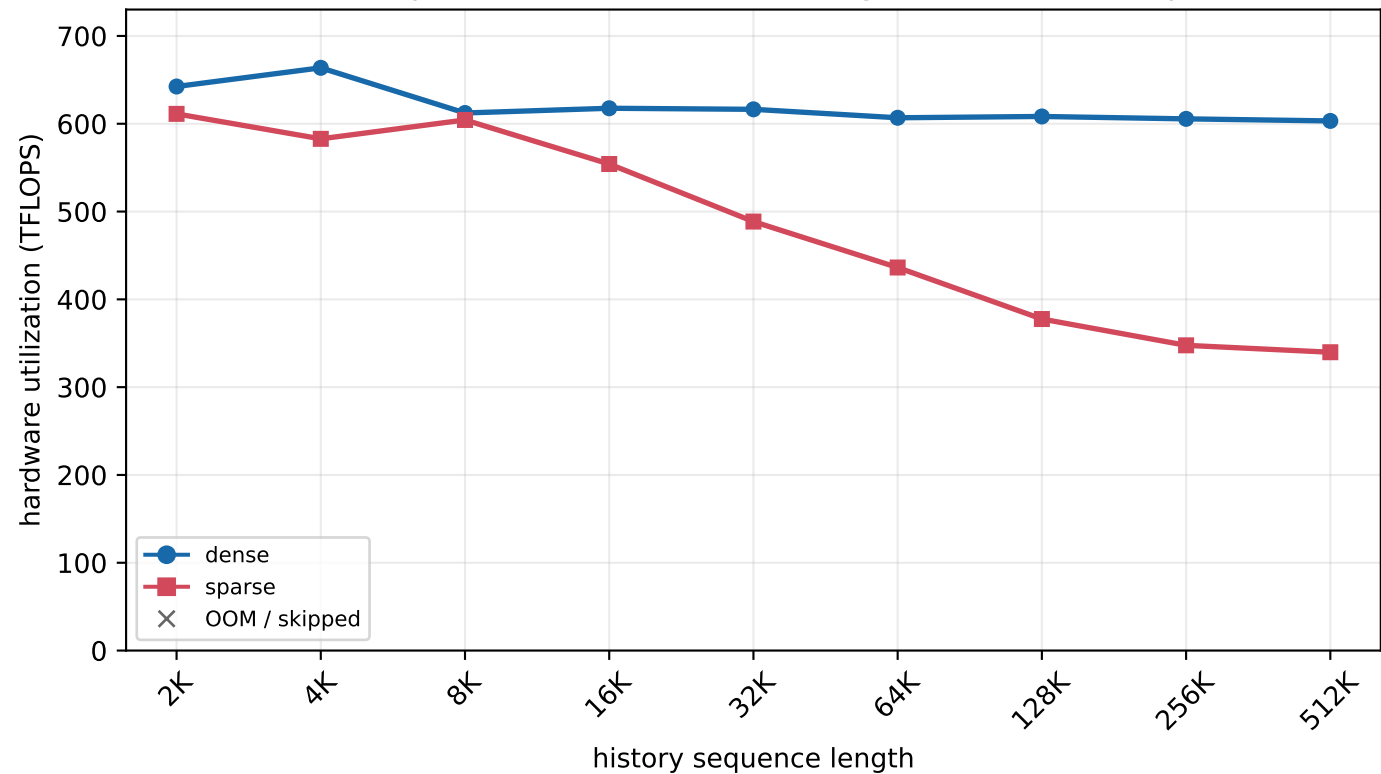
H800 MLA prefill - batch=128, new length=128 (chunked prefill)
