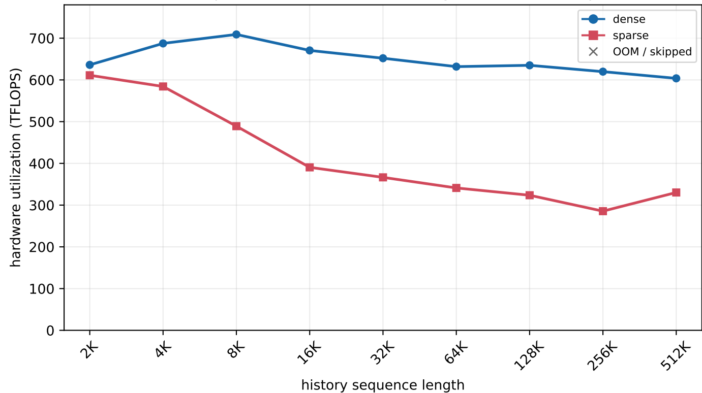
H800 MLA prefill - batch=128, new length=16 (chunked prefill)
