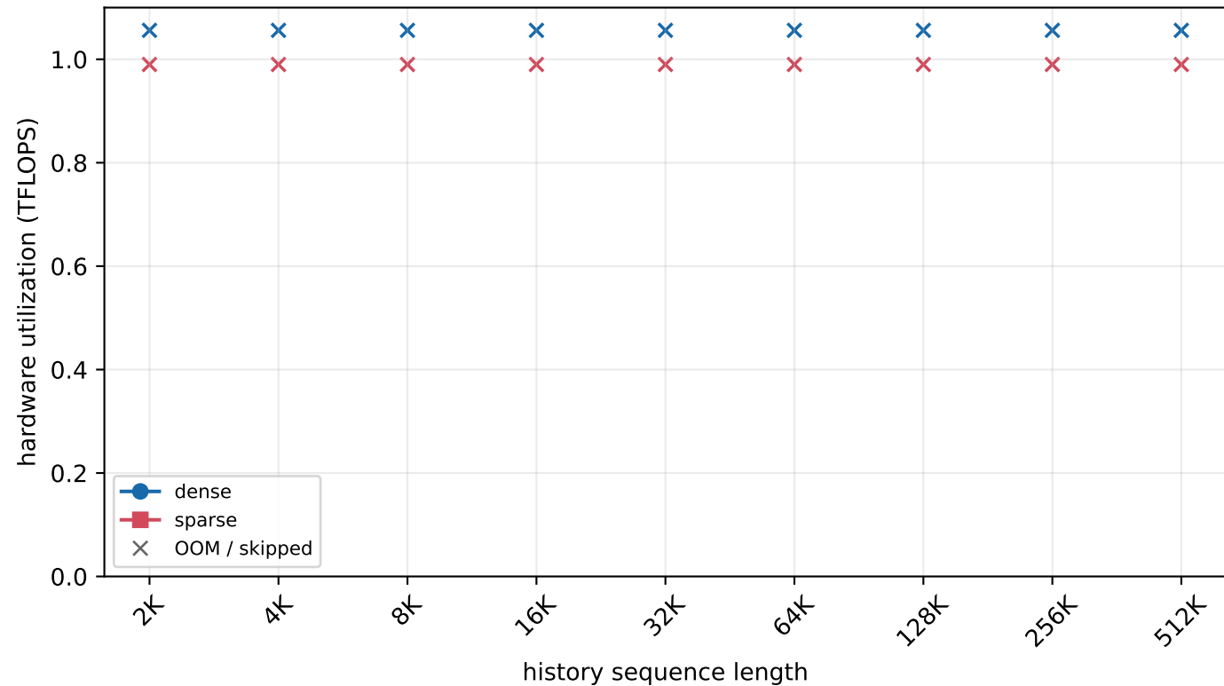
H800 MLA prefill - batch=128, new length=16K (chunked prefill)
