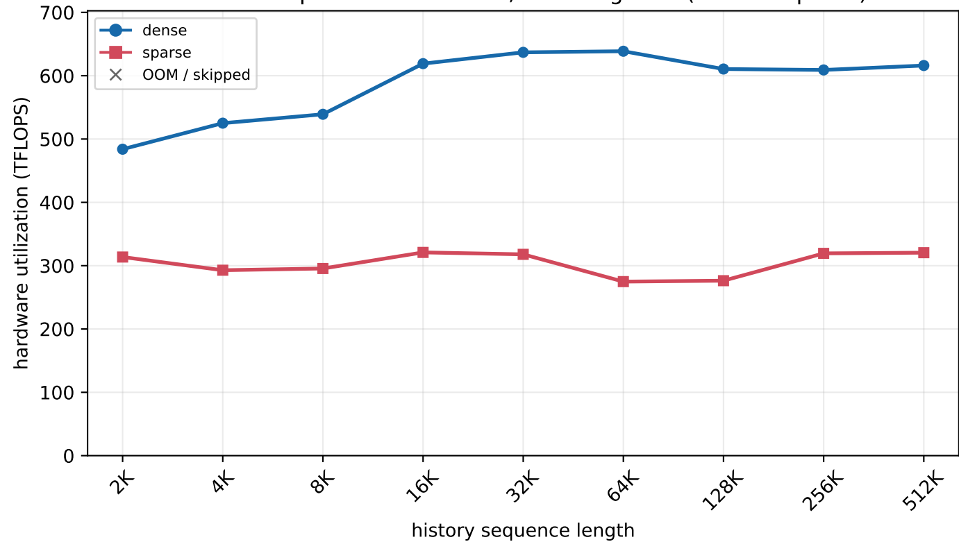
H800 MLA prefill - batch=128, new length=2 (chunked prefill)
