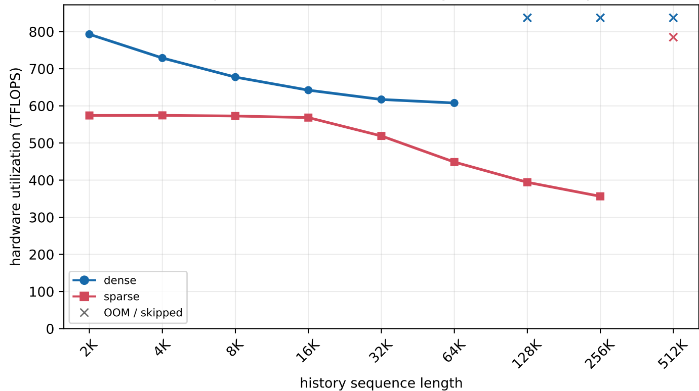
H800 MLA prefill - batch=128, new length=2K (chunked prefill)
