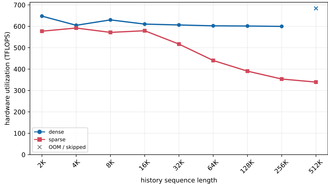
H800 MLA prefill - batch=128, new length=256 (chunked prefill)
