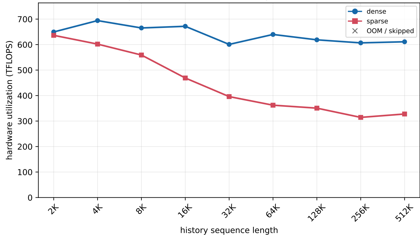
H800 MLA prefill - batch=128, new length=32 (chunked prefill)
