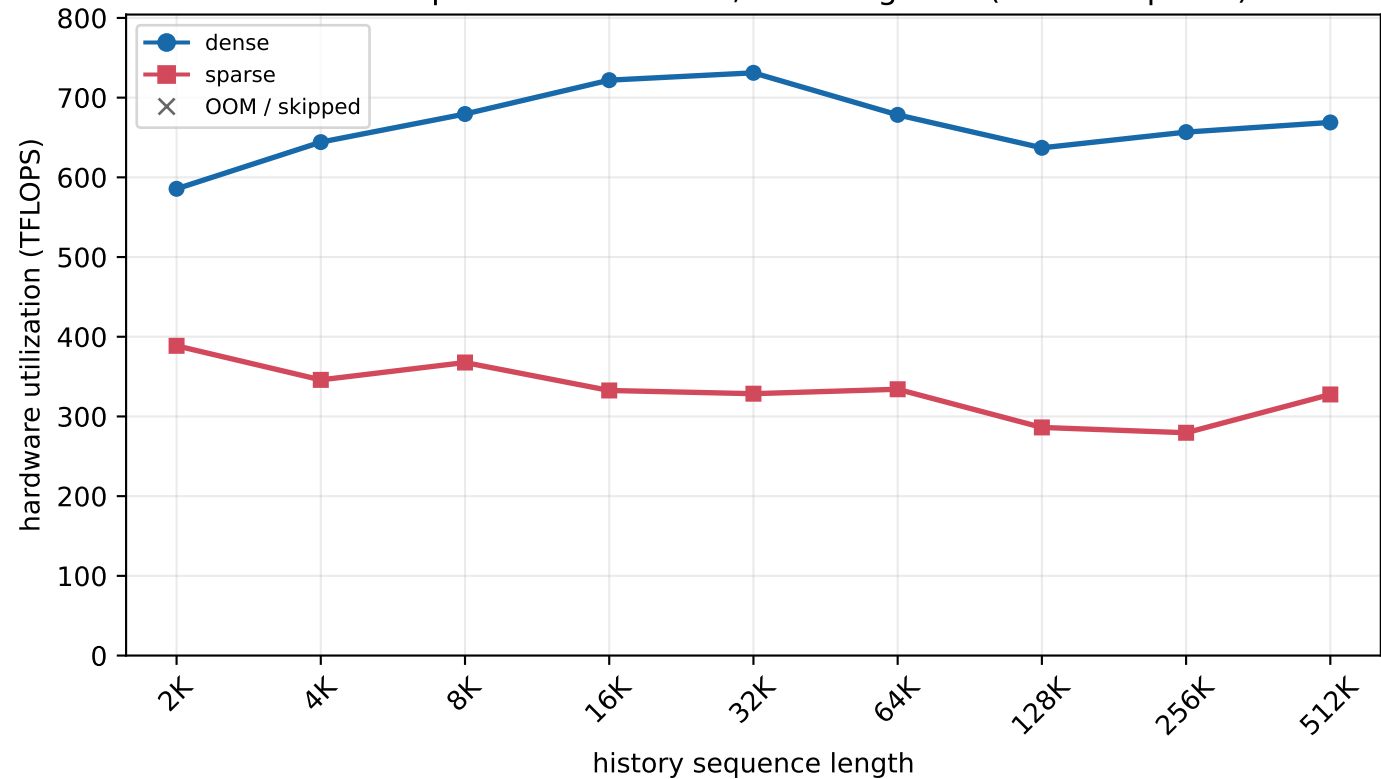
H800 MLA prefill - batch=128, new length=4 (chunked prefill)
