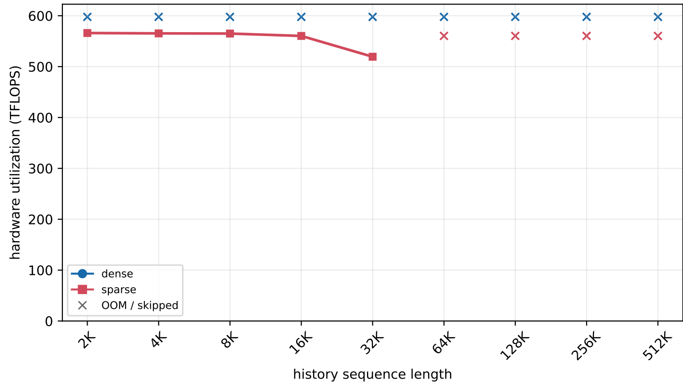
H800 MLA prefill - batch=128, new length=4K (chunked prefill)
